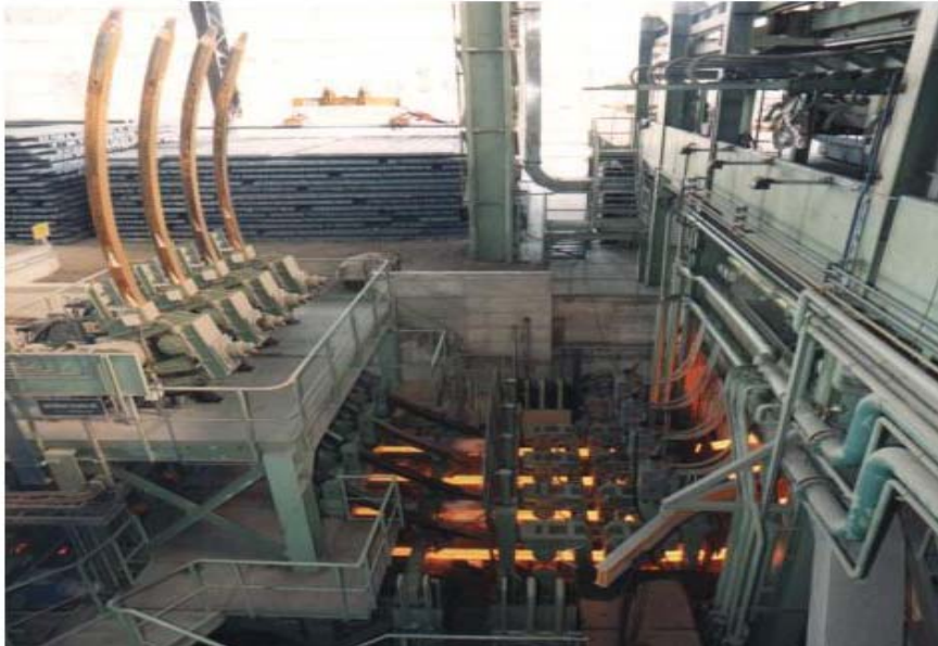
1994 FERALPY (GERMANY) BILLET CONTINUOUS CASTING MACHINE
