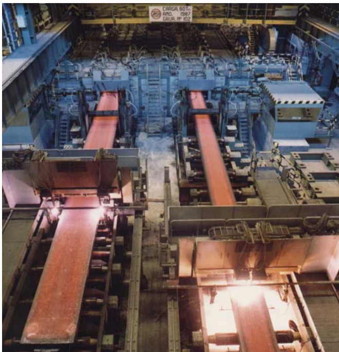
1988 ENSIDESA (SPAIN) CONTINUOUS CASTING PLANT
